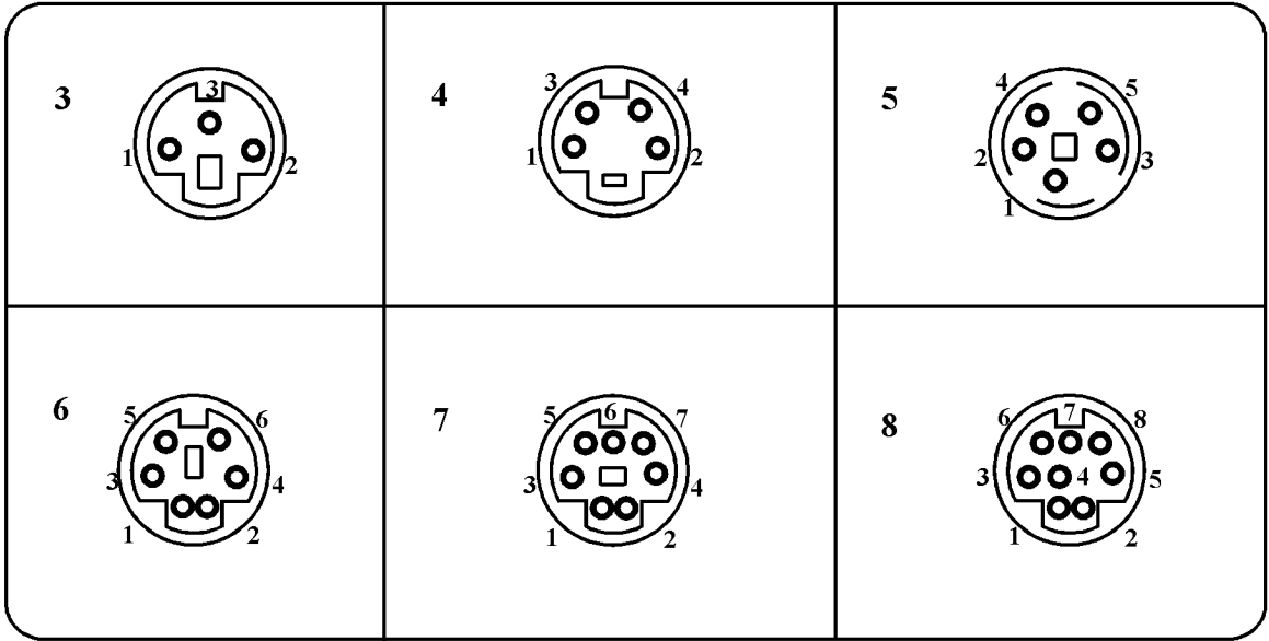
Contact Layout (Facing View)
