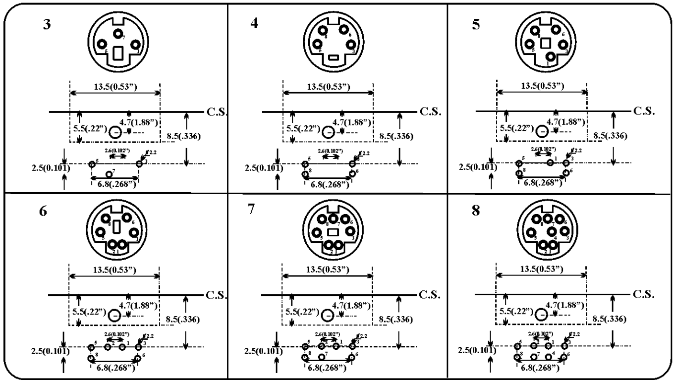
PCB LAYOUT (Component Bottom View)
